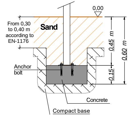
FOUNDATION DETAIL for sandbox
